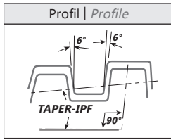
Extreme-Line Casing
