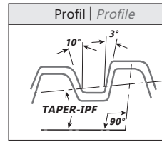
Buttress Casing
